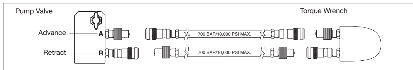
Figure 5, Hose Details (top view)
