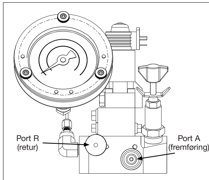
Figur 4, Ventilcuplinger
