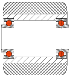
ZZV-Rillenkugellager
