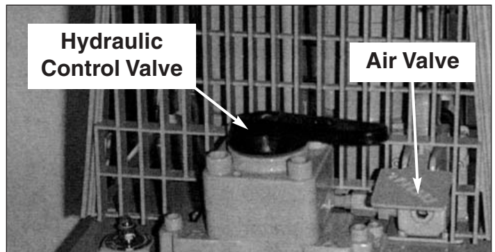
Figure 6 - Pump Controls
